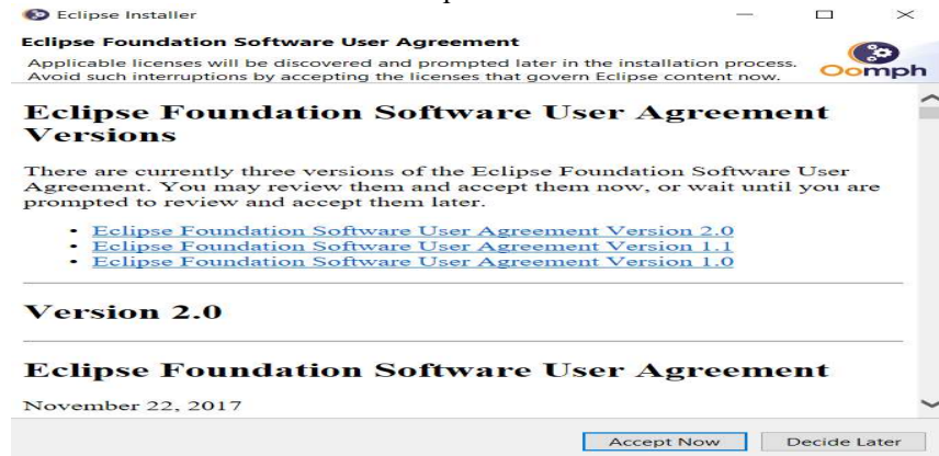
Figure 14: User Agreement
