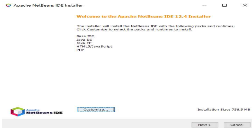
Figure 2.7: Installer Wizard
