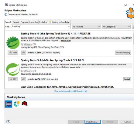
Figure 2.38: Eclipse Marketplace
