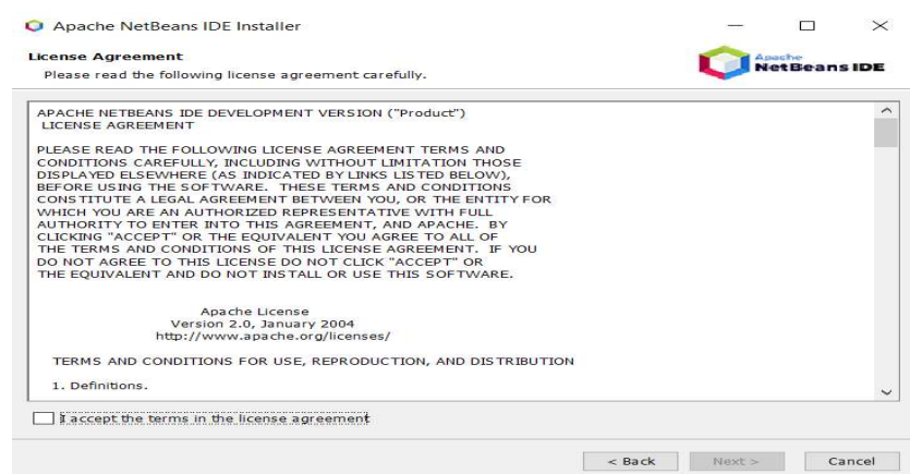
Figure 2.8: License Agreement
