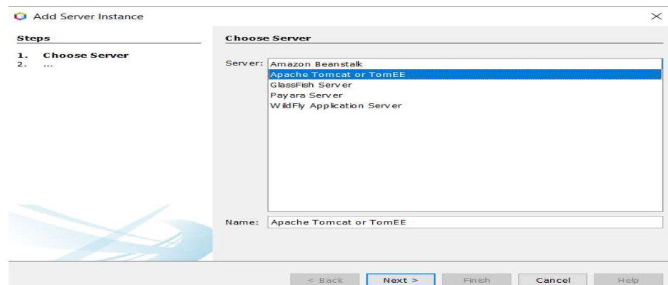
Figure 2.24: Server Selection
